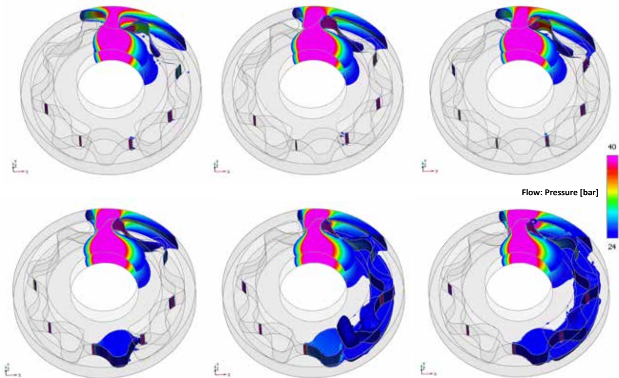
Fig. 6 CFD is used to identify the high pressure zone in this gerotor simulation
